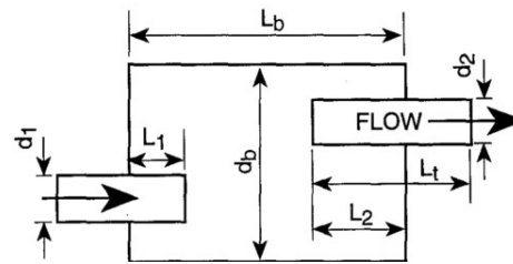
Illustration 6: Re-entrant diffusion muffler, Blair
