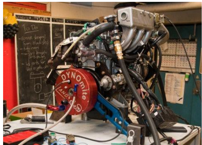
Illustration 2: T660 engine attached to dynamometer
