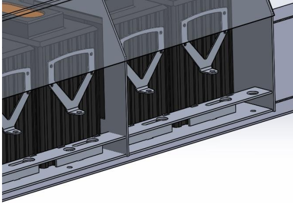
Figure 5: Slots and tabs are used for easy assembly and welding.
