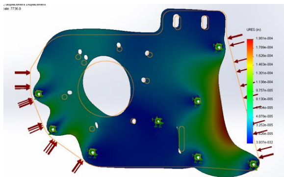
Figure 3: SolidWorks exaggeration of displacement of the structure.
