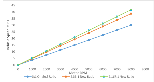
Figure 10: Plot shows the relation between motor speed and rpm with various belt ratios.
