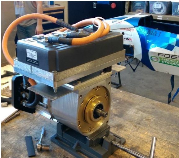
Figure 8: Motor and controller assembly.
