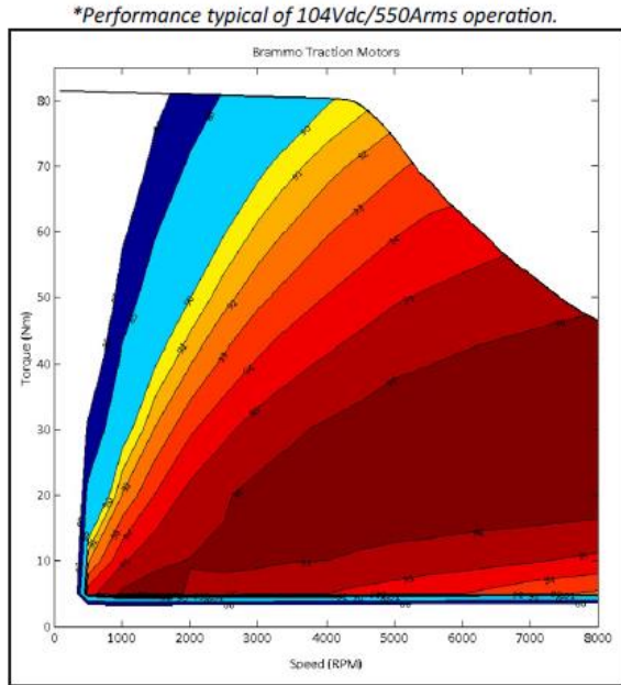
Figure 11: Torque curve of the Parker/Brammo Motor. Peak torque is represented by solid the line at top of curve.
