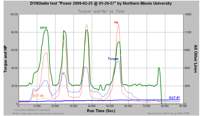
Figure A-8: Multiple Attempts to reach Max. Horsepower
