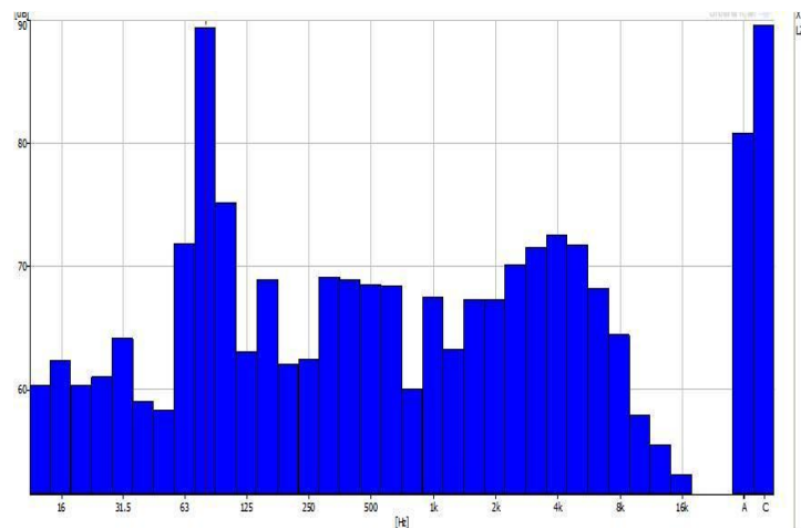
Figure A-6: dB (Vertical Axis) vs. Hz (Horizontal Axis) at 70-90 Hz, dB levels reached almost 90 dB.
