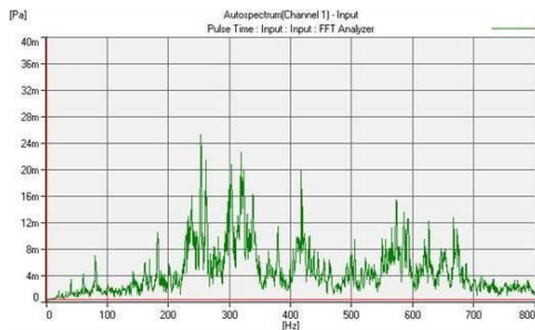
Figure 8. Spectrum analysis with stock muffler at idle
