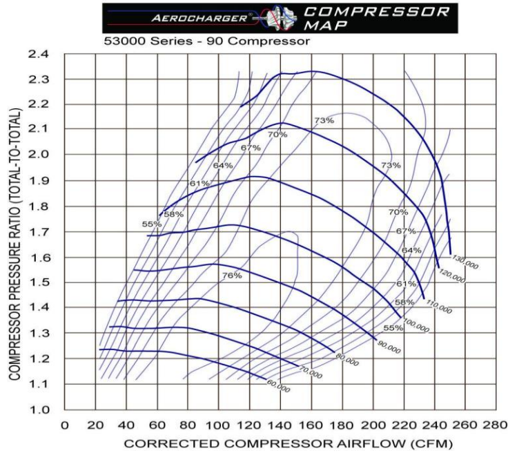
Figure A-9: Compressor Map for the Team's Turbocharger
