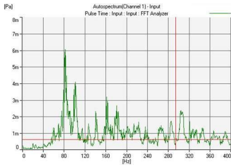
Figure 8. Spectrum analysis with stock muffler at idle
