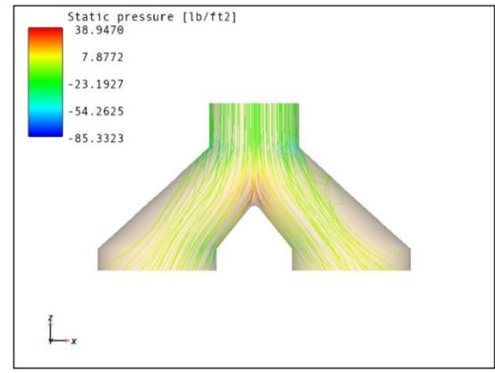
Figure 7: Flow Analysis through Throttle Body Inlet
