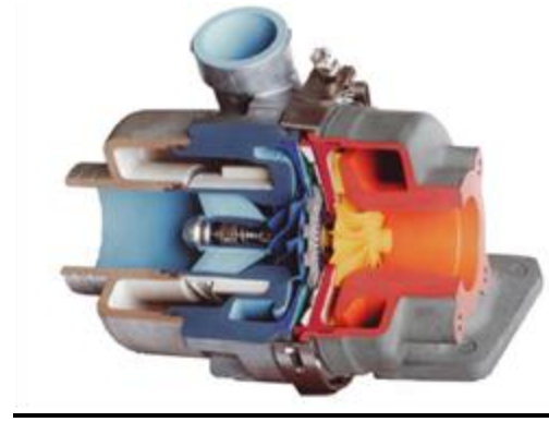
Figure 4: Section View of the Aerocharger Turbo
