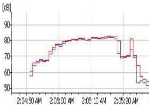
Figure A-5: dB Level at Mid Throttle from 50ft. Away
