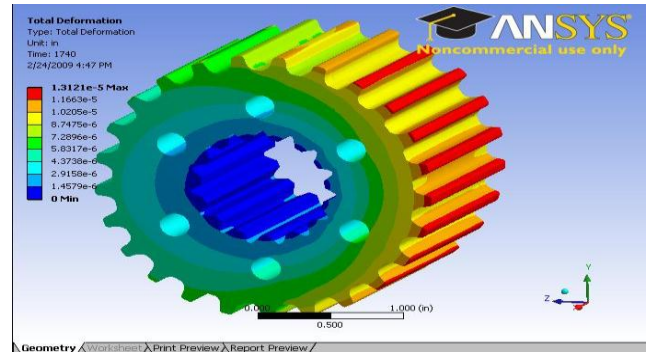
Figure A-3: Total Deformation on Small Gear
