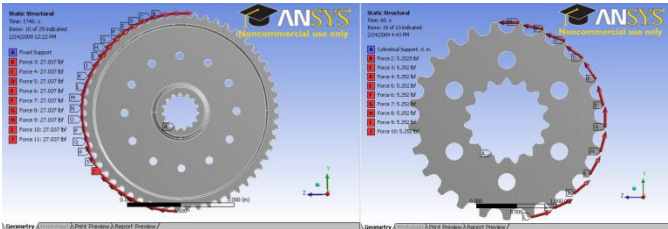
Figure 6: Forces Applied to Large and Small Gear
