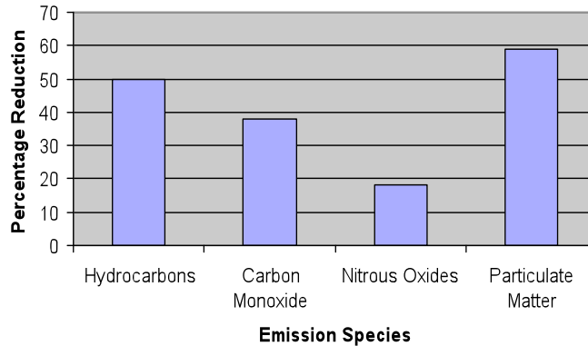
Figure 1 Reduction in Snowmobile Engine Emissions Using E85 Compared to Gasoline [3]
