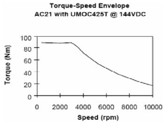
Figure 9 - Motor Torque-Speed Envelope
