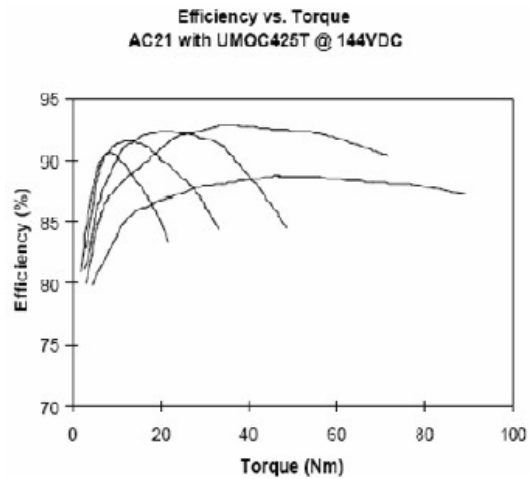
Figure 10 - Motor efficiency graph
