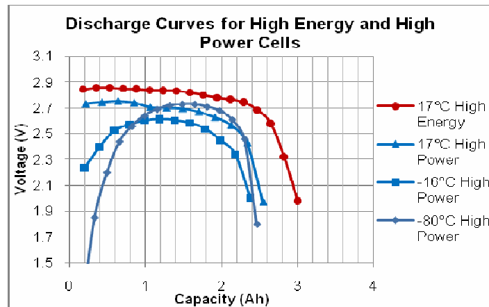
Figure 2 - Discharge curves of both High Energy and High Power K2 Cells. High Power Cells were also discharged under different temperature conditions. Note that the -80°C data is for cells that were soaked in -80°C and then discharged at -1°C due to equipment limitation
