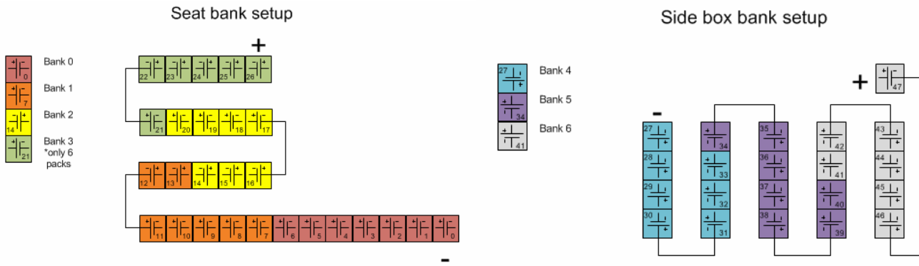
Figure 4 - BMS Bank Setup in Snowmobile
