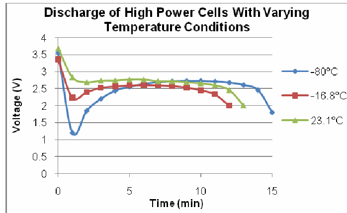
Figure 3 - voltage discharge of batteries in different ambient temperatures. (80°C denotes soak temperature discharge temperature was -1°C
